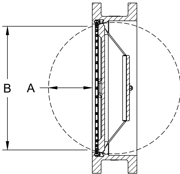
FLANGED
