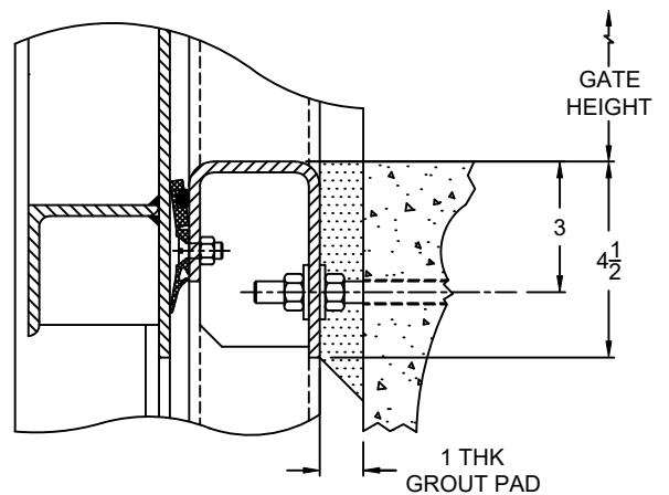
SECTION VIEW - B CROSS RAIL
