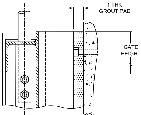
SECTION VIEW - C TOP OF SLIDE (RISING STEM)
