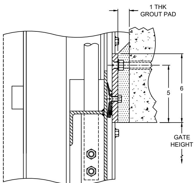
SECTION VIEW - C CROSS RAIL (STANDARD RISING STEM)
