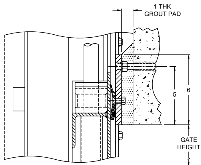
SECTION VIEW - C CROSS RAIL (OPTIONAL NON-RISING STEM)
