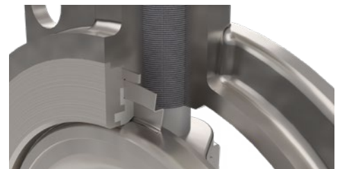
Optional Fire-Safe Seat
