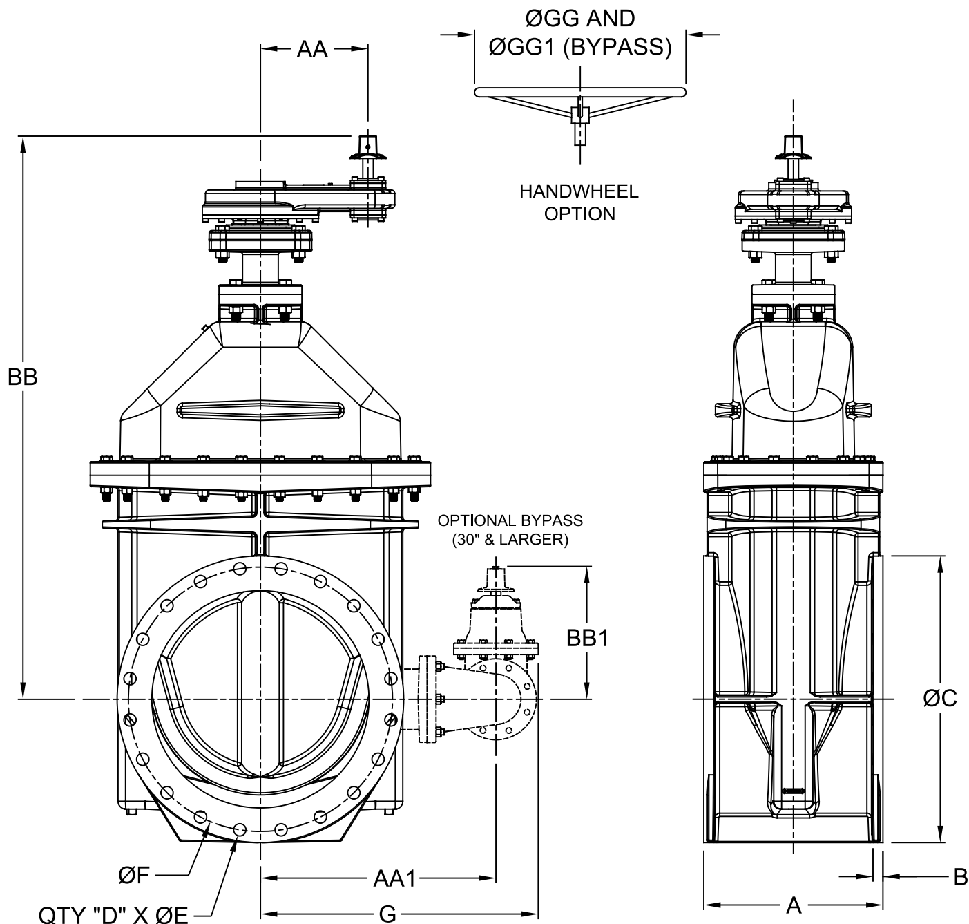
DIMENSIONS (Inches)
