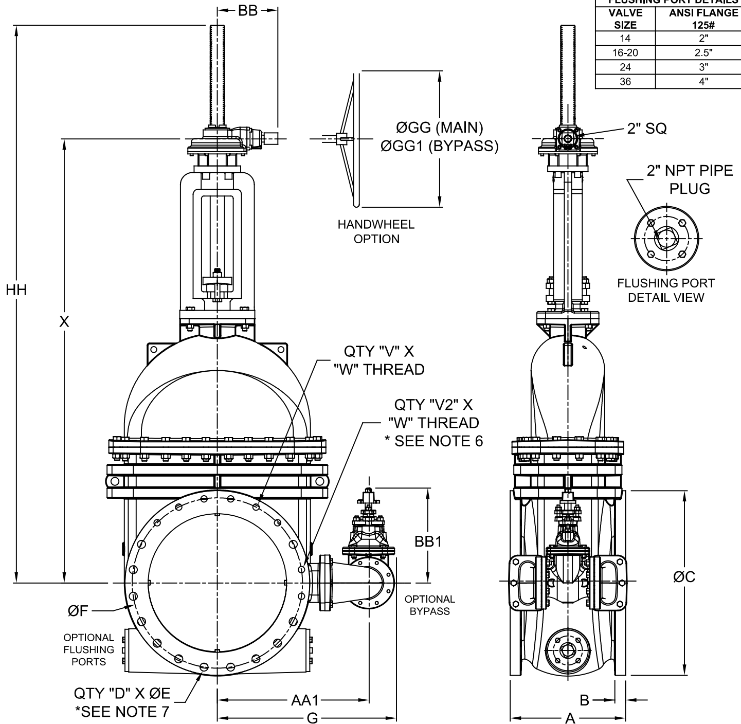
DIMENSIONS (Inches)
