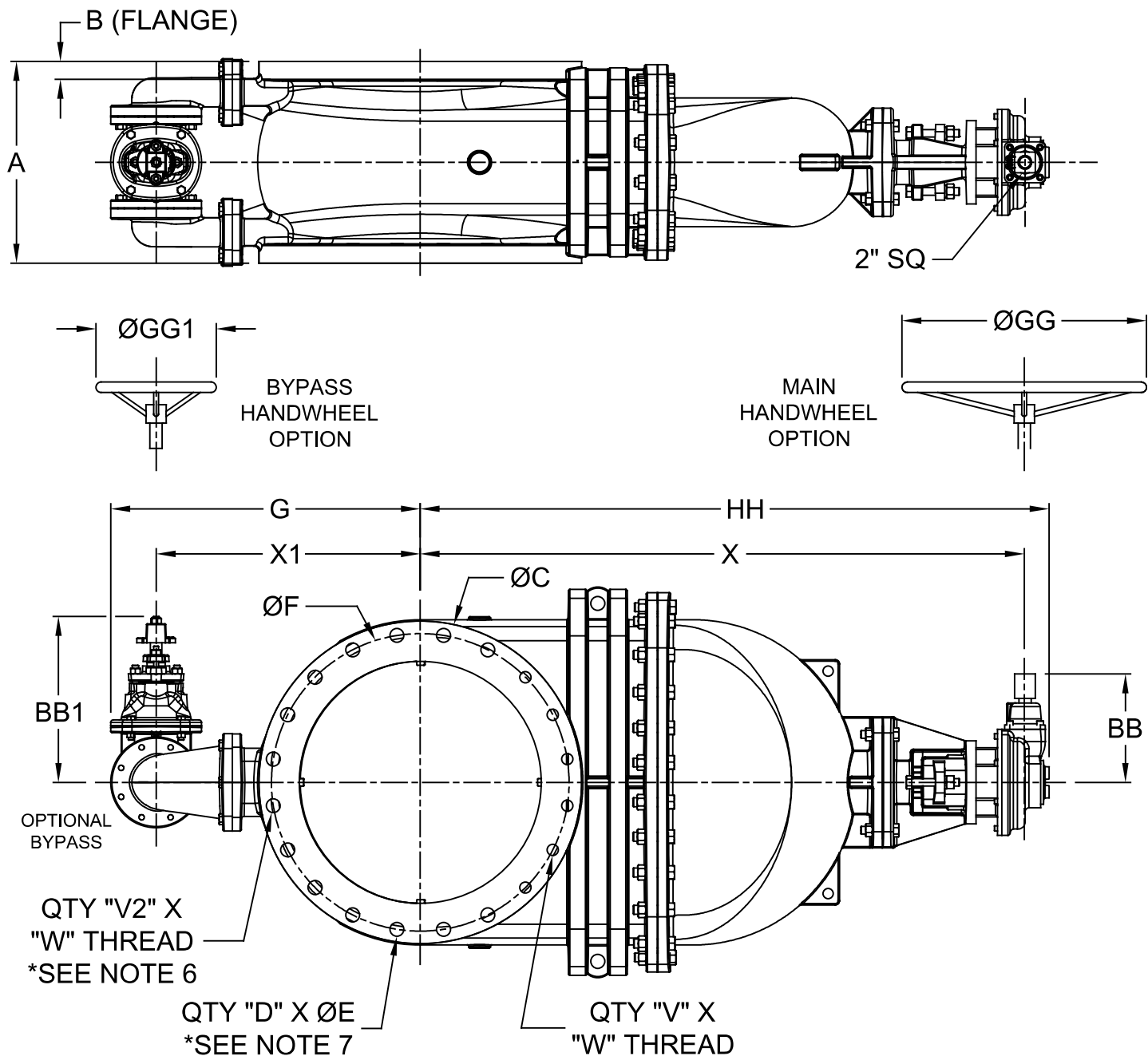
DIMENSIONS (Inches)
