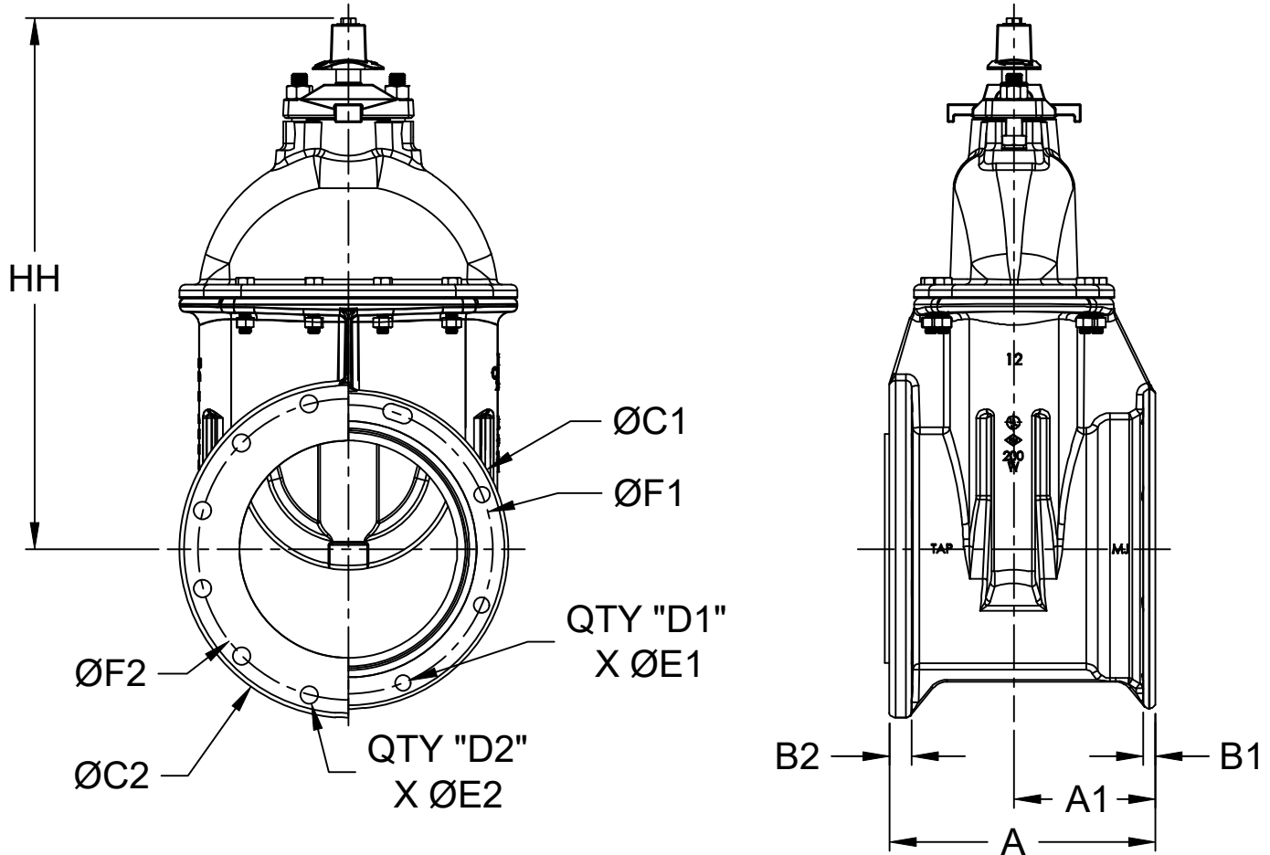
DIMENSIONS (Inches)
